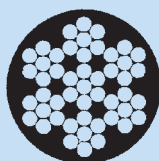
7x7 PVC/PP/PE
